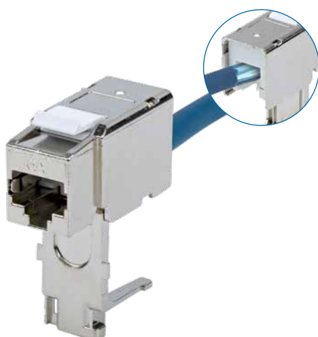
3 Fit to the front
