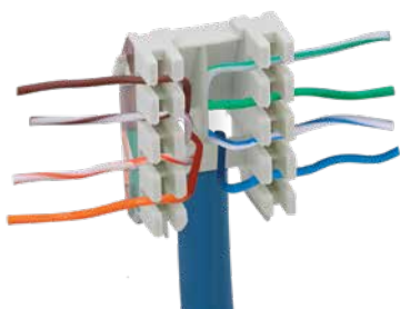
2 Separate and fit the pairs
